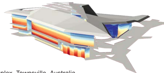
Parametric Roof Optimisation, JCU Technology Innovation Complex, Townsville, Australia
