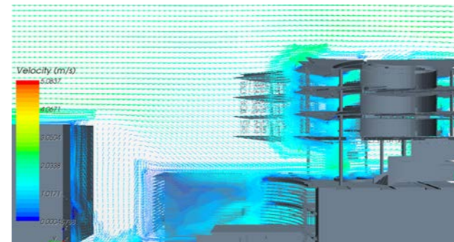
Ventilation Analysis, NTU 'The Arc', Singapore
