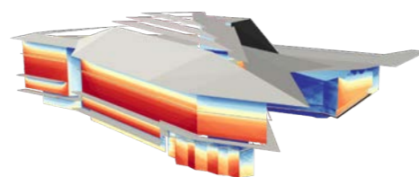
Parametric Roof Optimisation, JCU Technology Innovation Complex, Townsville, Australia
