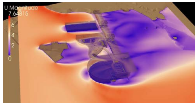
CFD Analysis, NTU 'The Arc', Singapore
