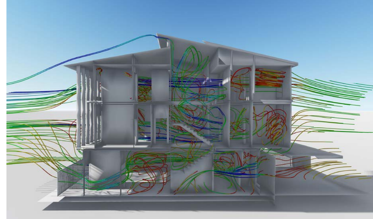
Cyberjaya South Apartments CFD Analysis, Cyberjaya South, Malaysia
