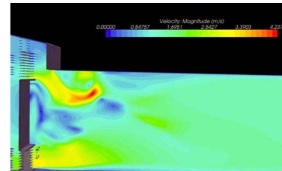
Ventilation Analysis, NTU 'The ARC', Singapore
